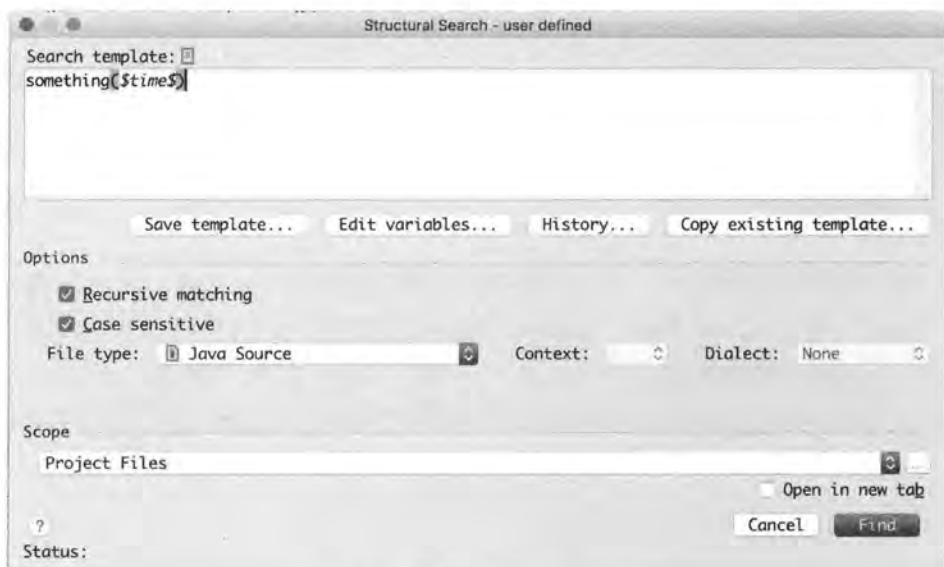
图 3.59 Structurally Search
