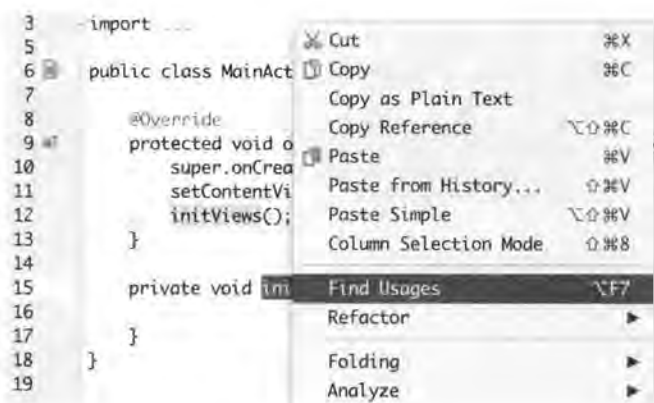
图 3.18 Find Usages
