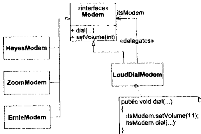
图 28.5 DECORATOR: LoudDialModem
