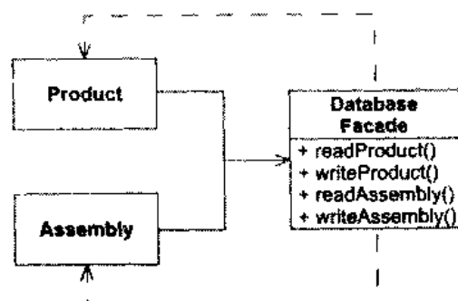
图 26.10 Database Facade
